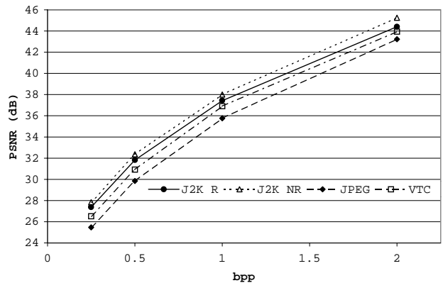
Figure 1: PSNR corresponding to average RMSE, of all test images, for each algorithm when performing lossy encoding at 0.25, 0.5, 1 and 2 bpp.
